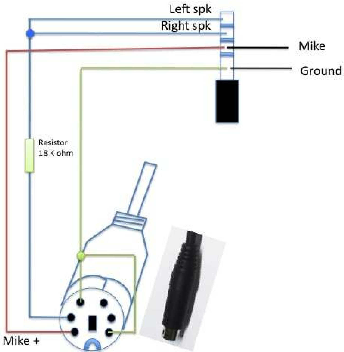
Male plug, view from out side
